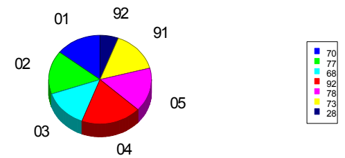
Class Distribution
